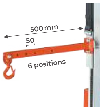
E/POTENCE • Crochet
